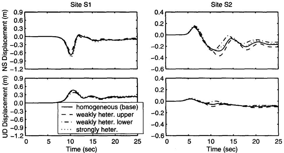
Figure 22. Comparison of north-south and vertical displacement time histories at sites S1 and S2 for the four slip distributions.
