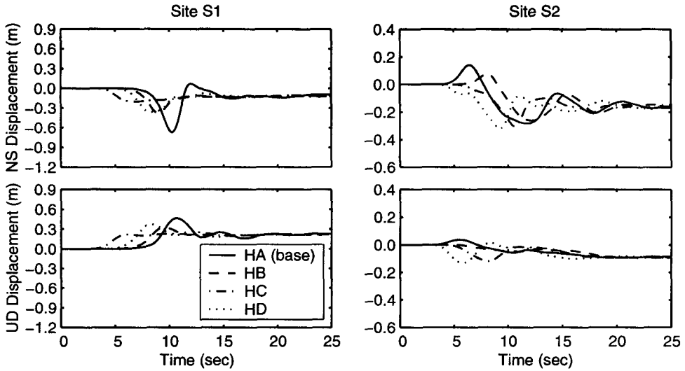
Figure 21. Comparison of north-south and vertical displacement time histories at sites S1 and S2 for the four hypocenter locations.
