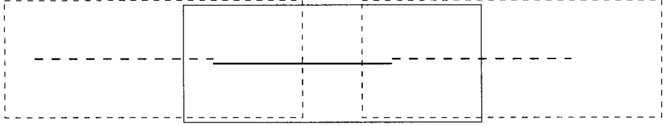
Figure 25. Diagram showing the construction of an infinitely long fault composed of identical strike-slip fault domains with the faults lying end to end. The solid lines identify the original domain, and the dashed lines identify domains (with a slight offset for clarity) added to each end to extend the fault. We compile distributions of the maximum displacement and velocity as a function of distance from the infinitely long fault by selecting the maximum values from the overlapping distributions of the displacements and velocities associated with each domain.
