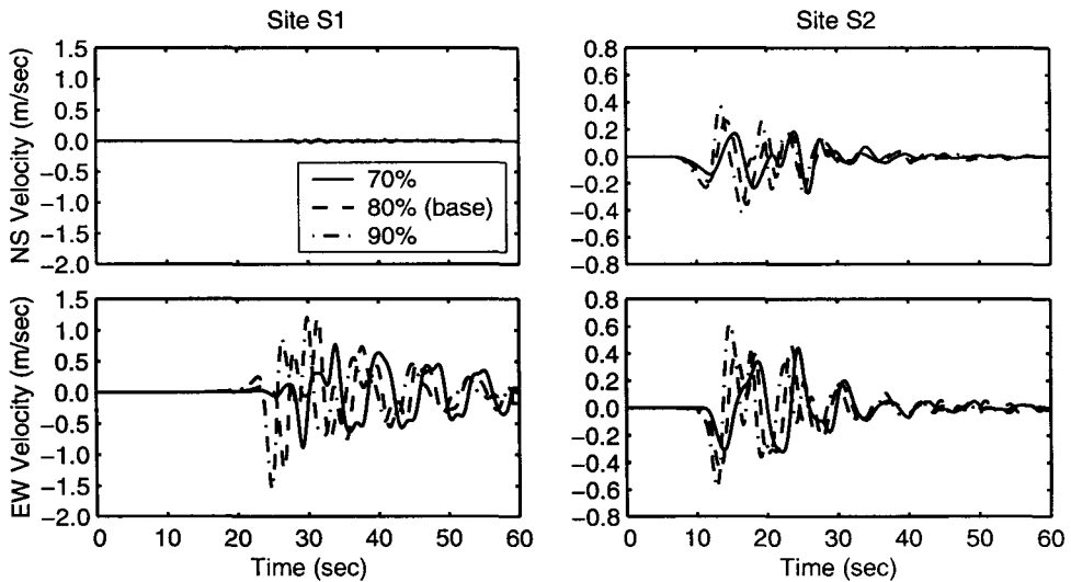
Figure 10. Comparison of horizontal velocity time histories at sites S1 and S2 for the three rupture speeds.
