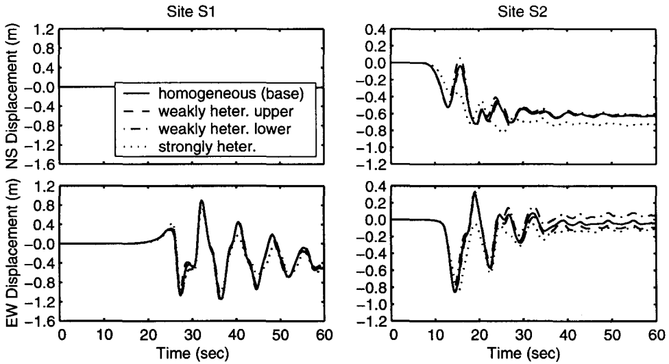
Figure 12. Comparison of horizontal displacement time histories at sites S1 and S2 for the four slip distributions.
