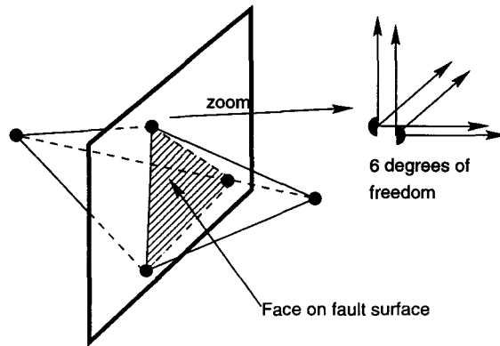
Figure 1. Model of the fault plane in the finite-element mesh. The left portion shows the alignment of the elements on the fault plane. The right portion provides a close-up of a node and its six translational degrees of freedom which allow the sides of the fault to move relative to each other.
