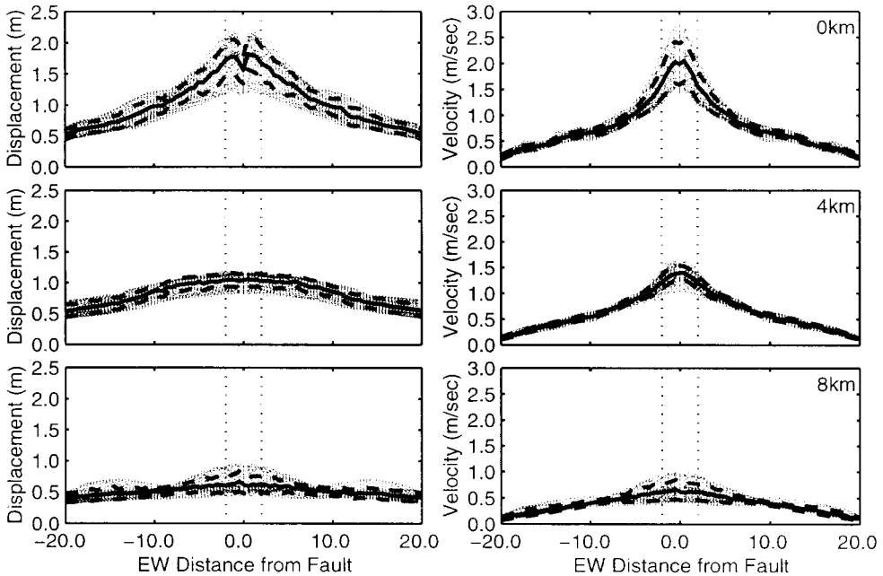
Figure 26. Maximum horizontal displacements and velocities on the ground surface as a function of distance from the surface projection of the top edge of the strike-slip fault for the three fault depths. The thick lines display the average and plus or minus one standard deviation. The vertical, dotted lines bound the zone with the highest near-source factor from the 1997 UBC .
