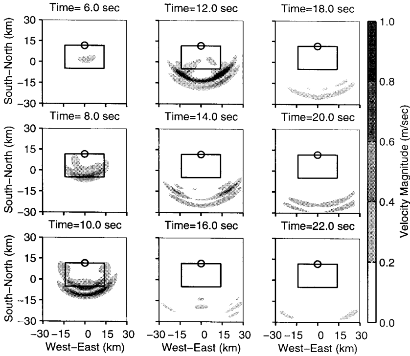
Figure 16. Snapshots of the magnitude of the velocity vector (0.5Hz low-pass filtered) at each point on the ground surface for scenario base. The solid line indicates the projection of the fault onto the ground surface, and the hollow circle identifies the epicenter. The south-southeast slip direction (rake angle of 105°) creates the asymmetry in the east-west direction.
