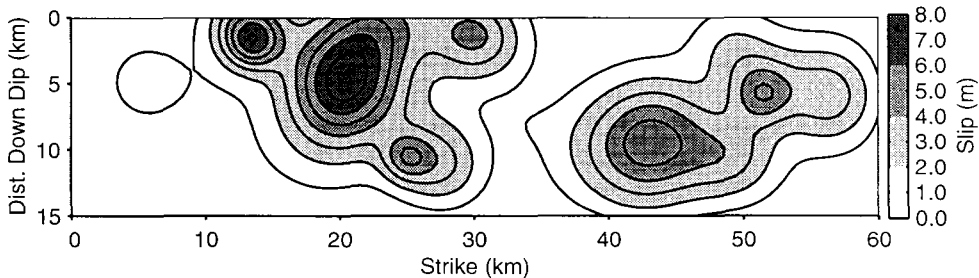
Figure 6. Strongly heterogeneous slip distribution strongheter, which is tapered on three edges with an average slip of 2.0 m and a maximum slip of 7.8 m.
