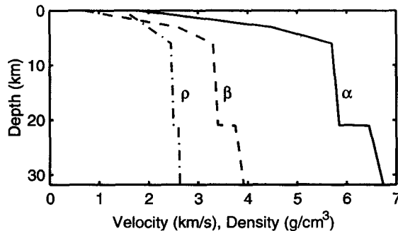
Figure 4. Density ( \rho ), shear-wave speed ( \beta ), and dilatational wave speed ( \alpha ) as a function of depth in the layered half-space.
