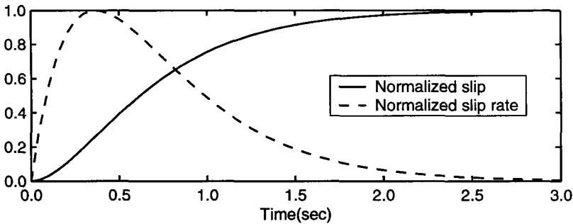
Figure 2. Slip and slip rate as a function of time for the Brune far-field time history function (shown for t_0 = 0 ).
