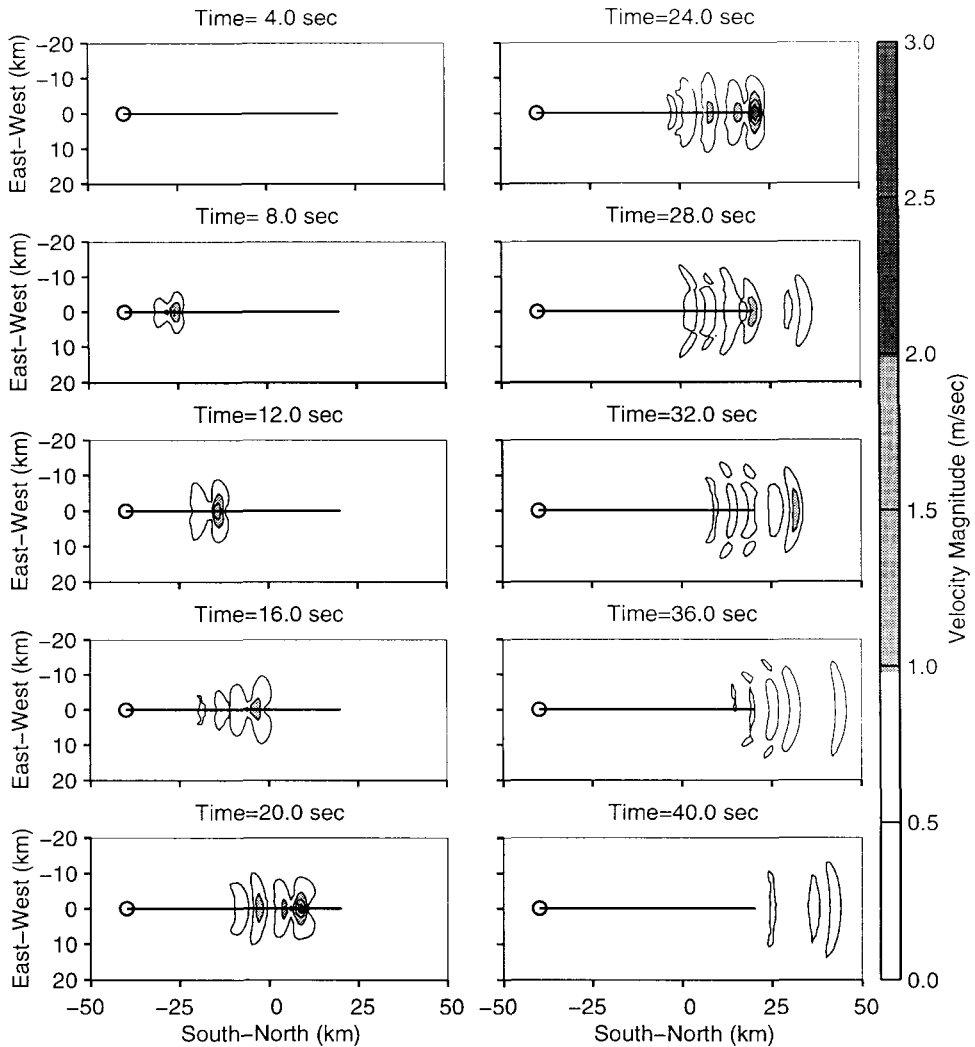
Figure 7. Snapshots of the magnitude of the velocity vector (0.5Hz low-pass filtered) at each point on the ground surface for scenario base. The solid line indicates the projection of the fault onto the ground surface, and the hollow circle identifies the epicenter.
