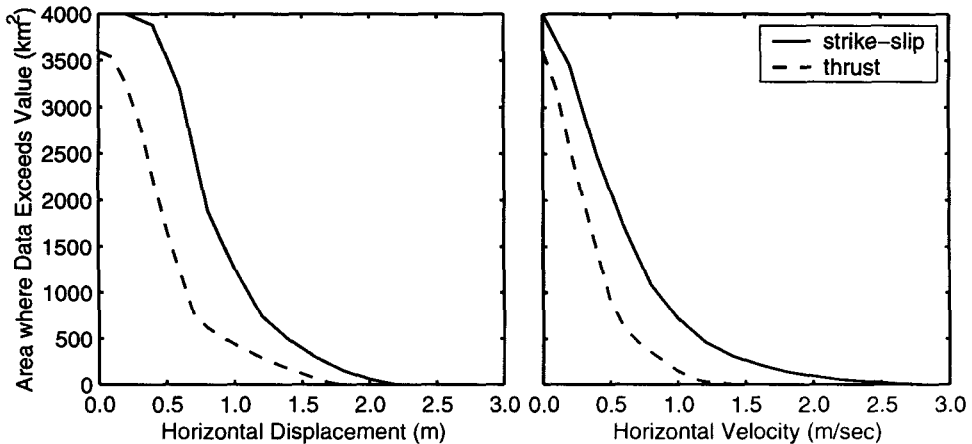
Figure 28. Areas on the ground surface in the strike-slip and thrust fault domains where the maximum horizontal displacements and velocities exceeded a given value.
