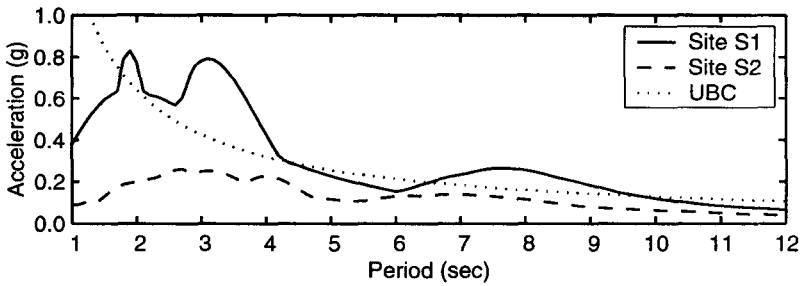
Figure 9. Horizontal acceleration response spectra for 5% critical damping at sites S1 and S2 for scenario base. The ground motions have been low-pass filtered to include periods greater than 2.0sec. The dotted line indicates the UBC design spectrum for a site with soil class S_D in zone 4 that lies within 2km of a fault designated as source type A.
