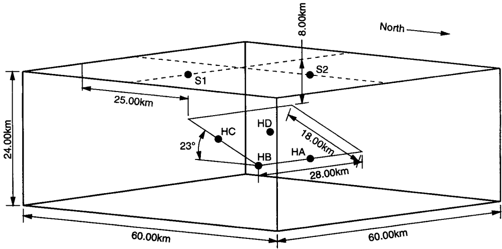
Figure 14. Domain geometry for the thrust fault for the case where the top of the fault lies 8.0 km below the ground surface. The labels HA through HD denote the various hypocenter locations. Waveforms are examined at site S1, which sits above the southeast corner of the fault, and site S2, which sits above hypocenter HA.
