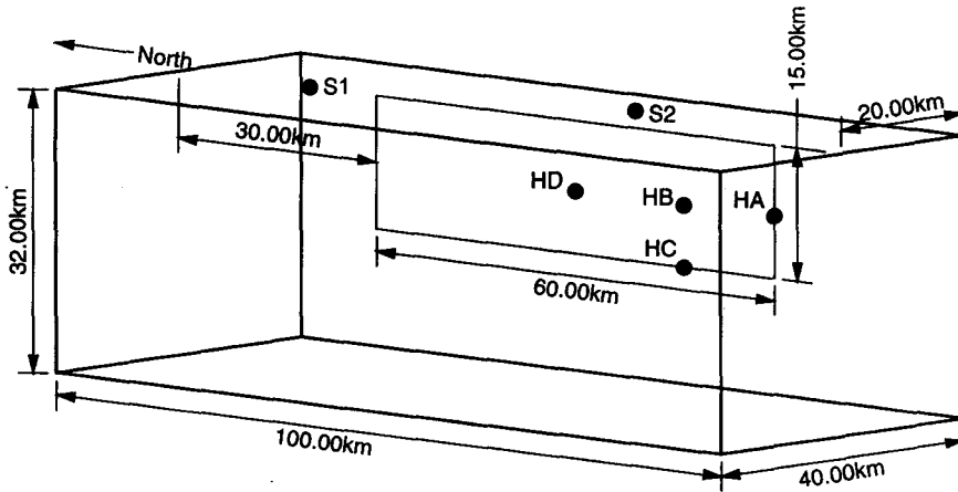
Figure 3. Domain geometry for the strike-slip fault for the case where the top of the fault reaches the ground surface. The labels HA through HD denote the various hypocenter locations. Waveforms are examined at sites S1 and S2.
