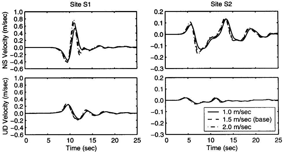
Figure 20. Comparison of north-south and vertical velocity time histories at sites S1 and S2 for the three peak slip rates.
