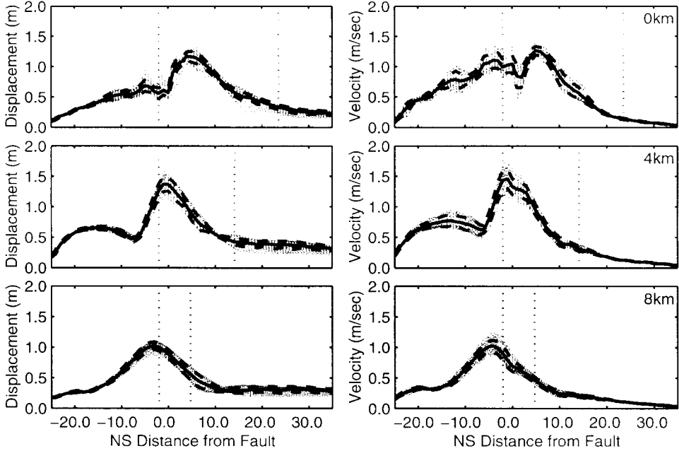
Figure 27. Maximum horizontal displacements and velocities on the ground surface as a function of distance from the surface projection of the top edge of the thrust fault for the three fault depths. The thick lines display the average and plus or minus one standard deviation. The vertical, dotted lines bound the zone with the highest near-source factor from the 1997 UBC .
