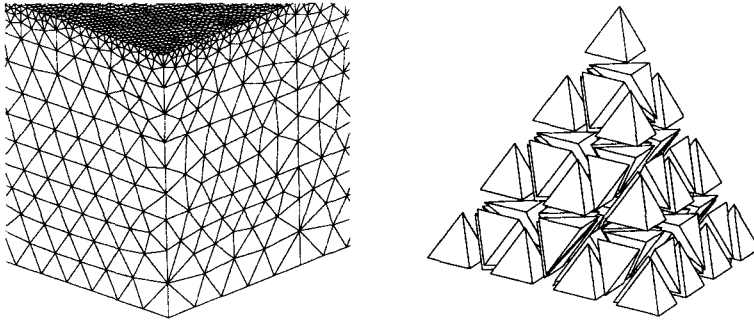
Figure 5. The plot on the left shows a corner of the coarse mesh, and the diagram on the right demonstrates how each element in the coarse mesh is divided into 64 elements to create the refined mesh.
