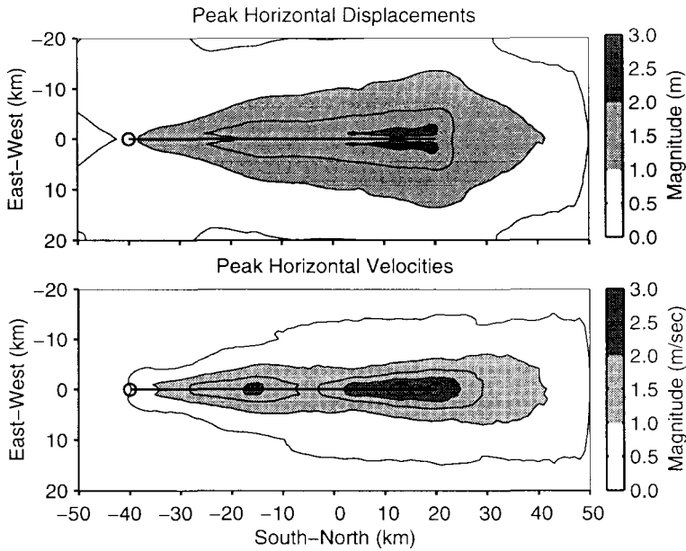
Figure 8. Maximum magnitudes of the horizontal displacement and velocity vectors (0.5 Hz low-pass filtered) at each point on the ground surface for scenario base. The solid line indicates the projection of the fault plane onto the ground surface, and the hollow circle identifies the epicenter.
