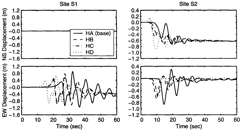
Figure 11. Comparison of horizontal displacement time histories at sites S1 and S2 for the four hypocenter locations.
