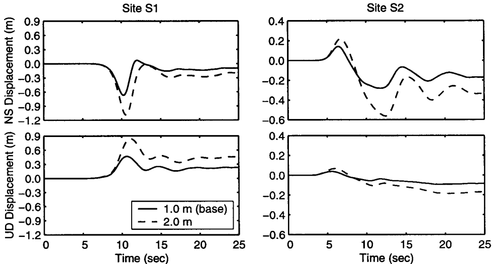
Figure 23. Comparison of north-south and vertical displacement time histories at sites S1 and S2 for the two values of average slip.
