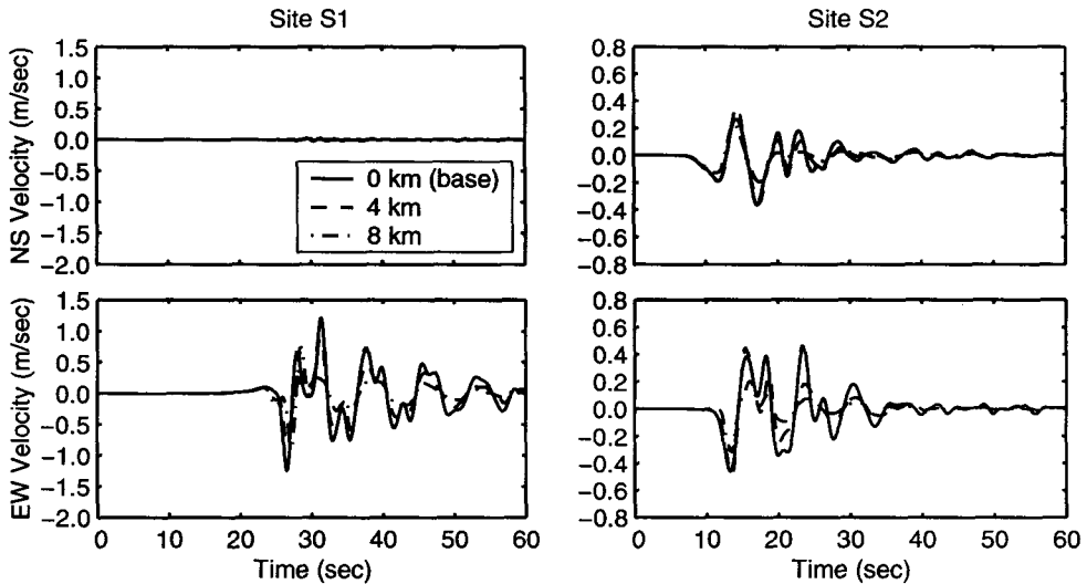
Figure 13. Comparison of horizontal velocity time histories at sites S1 and S2 for the three depths of the top of the fault.
