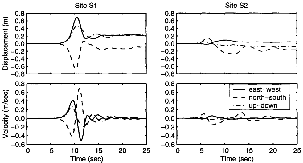
Figure 18. Displacement and velocity time histories at sites S1 and S2 for scenario base. Site S1 lies above the southeast corner of the fault, and site S2 lies at the epicenter.
