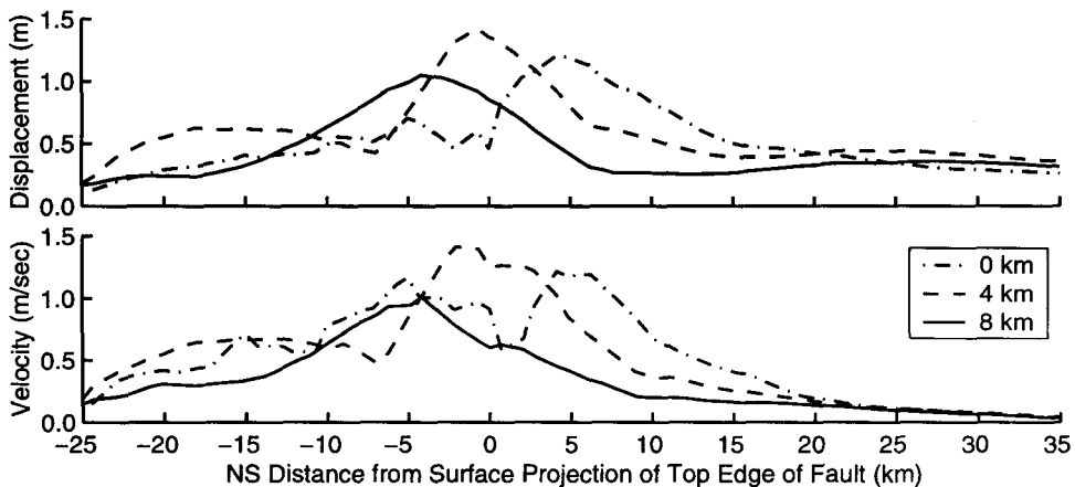
Figure 24. Maximum magnitudes of the horizontal displacement vectors and velocity vectors along a north-south line running over the center of the fault for the three depths of the fault.
