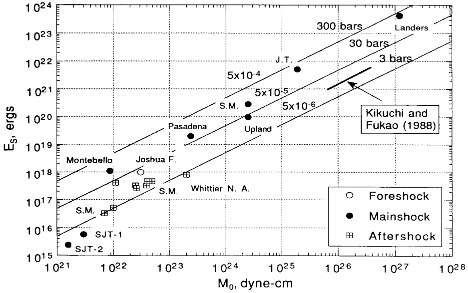
FIG. 6. The relation between seismic moment ( M_0 ) and energy ( E_S ). J.T.: Joshua Tree, S.M.: Sierra Madre, S.JT: San Jacinto Fault. The heavy solid line indicates the range of the E_S/M_0 ratios of large strike slip earthquakes determined by Kikuchi and Fukao (1988).
