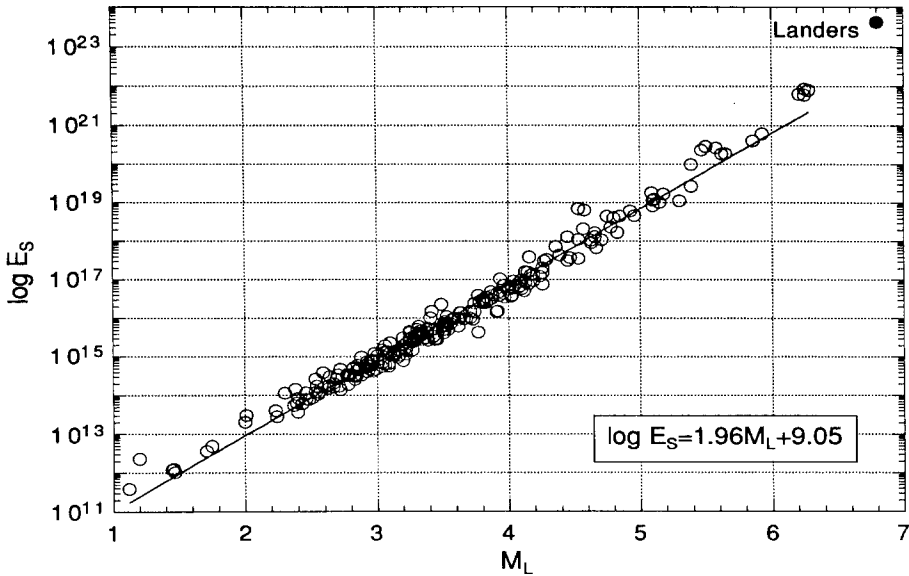
FIG. 5. The relation between \text{Log } E_S and M_L .
